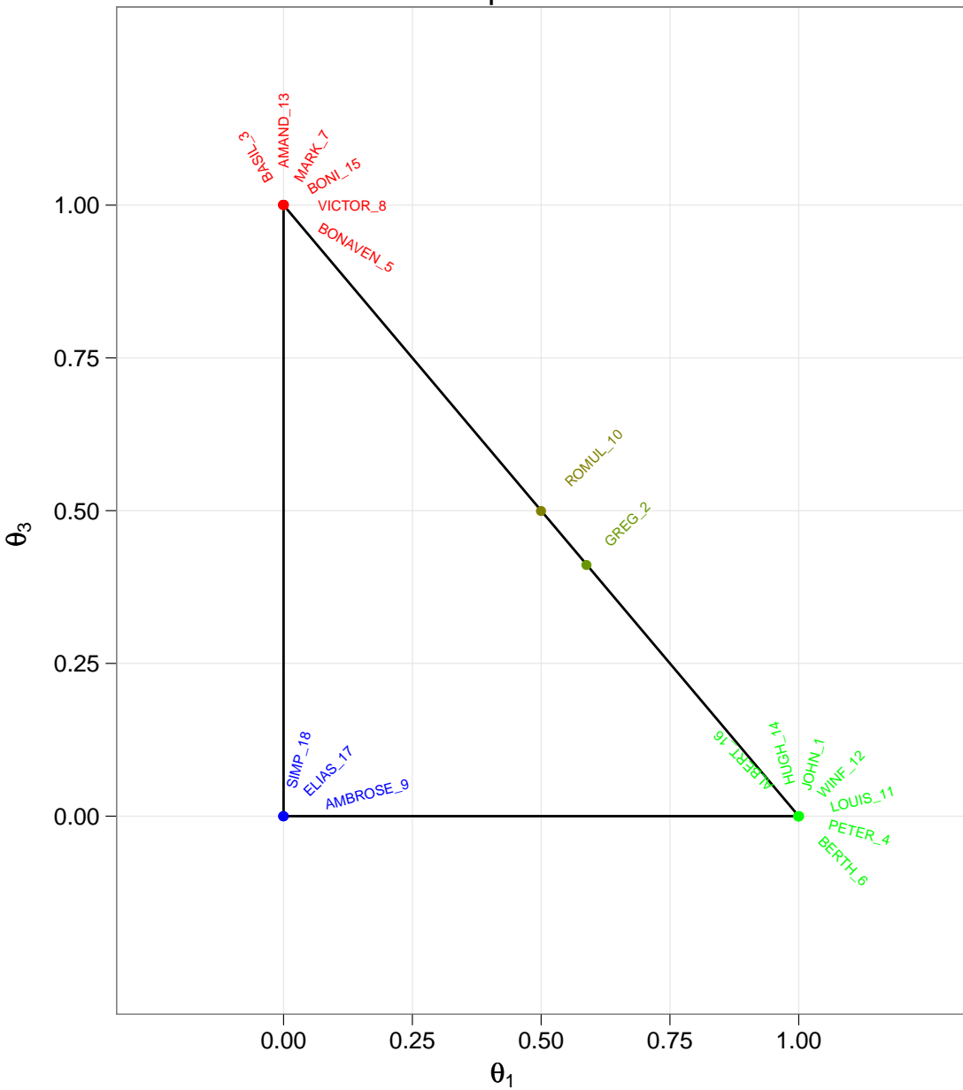
Latent positions
