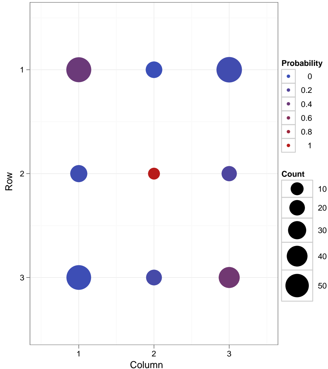
Block relations
