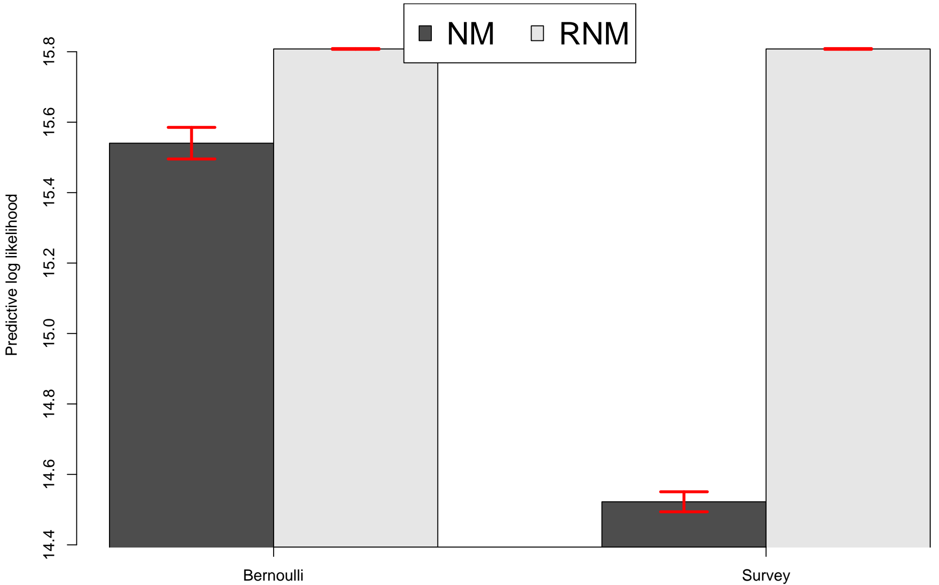
Two models on two holdout methods
